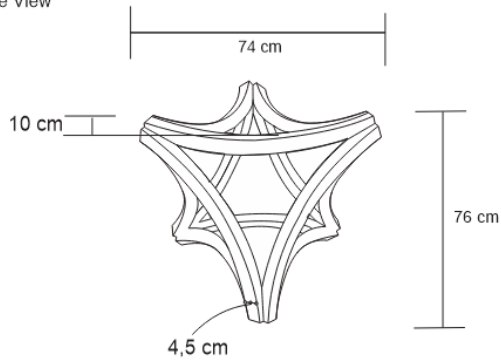
Base View
